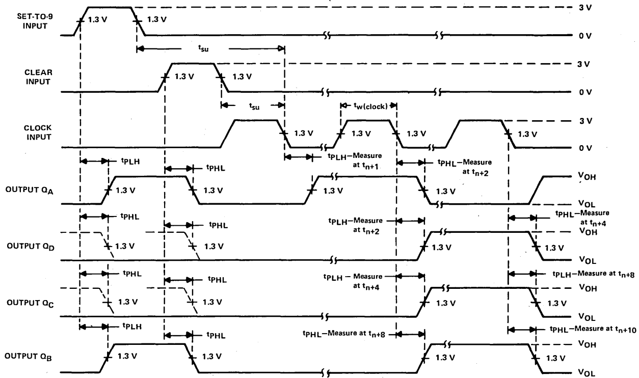
VOLTAGE WAVEFORMS
