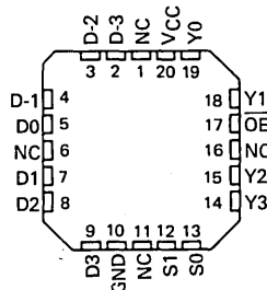
SN54S350 ... FK PACKAGE SN74S350 ... FN PACKAGE (TOP VIEW)
