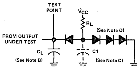
LOAD CIRCUIT
