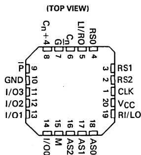
SN54LS681 ... FK PACKAGE SN74LS681 ... FN PACKAGE
