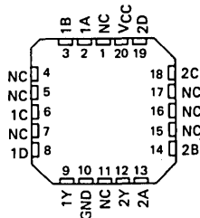
SN74LS19 ... FN PACKAGE
