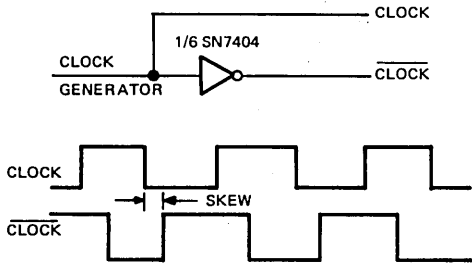
FIGURE A - TYPICAL CLOCK/CLOCK GENERATOR CIRCUIT
