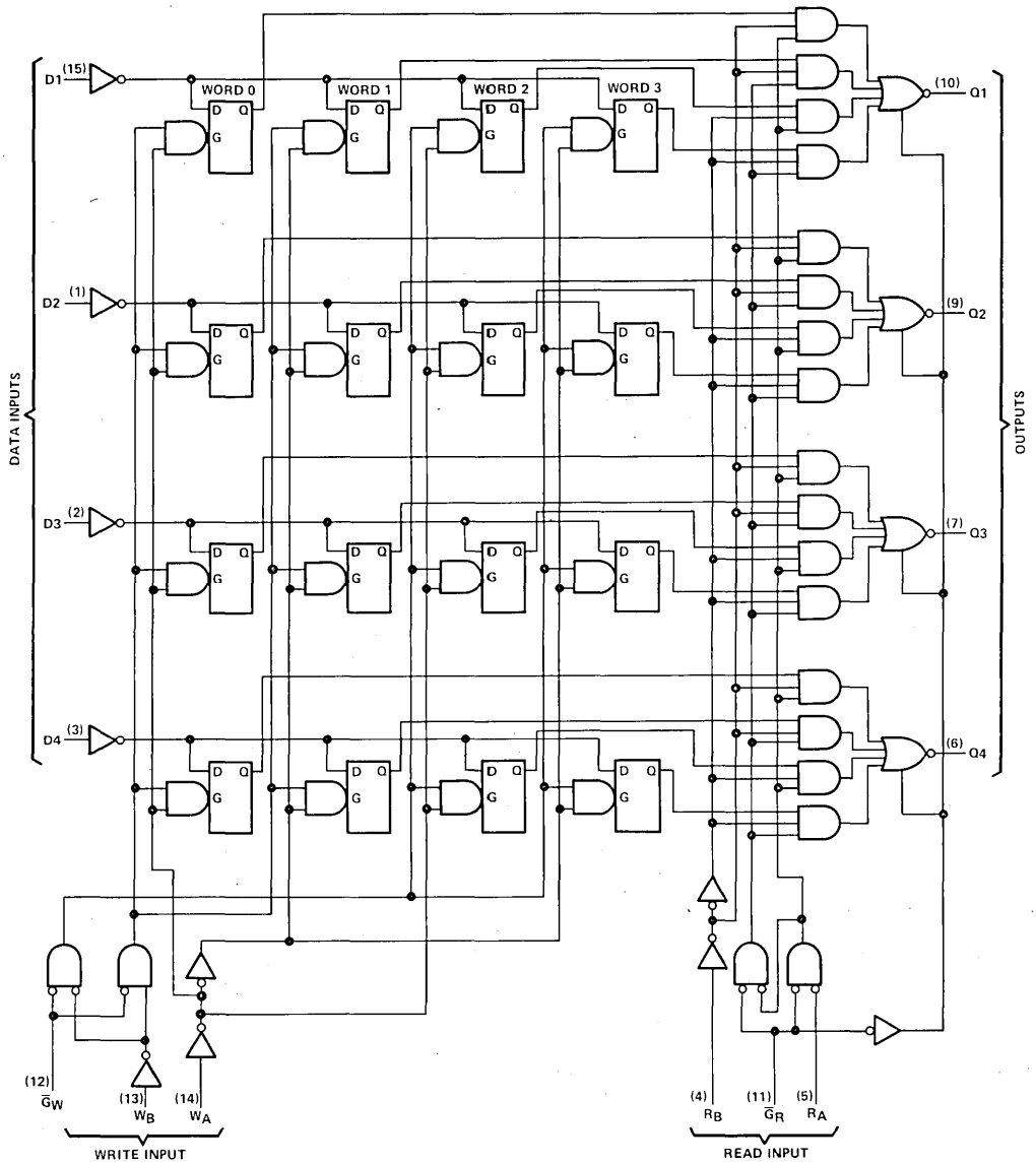
logic diagram
