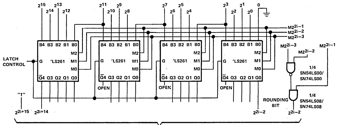
FIGURE A - FIRST PARTIAL PRODUCT, PP1
