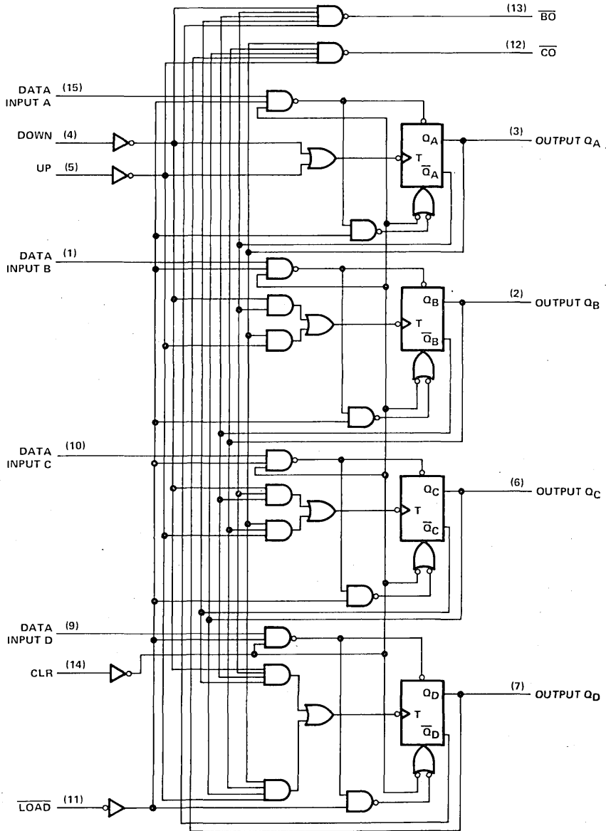
logic diagram
