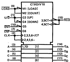
logic symbol
