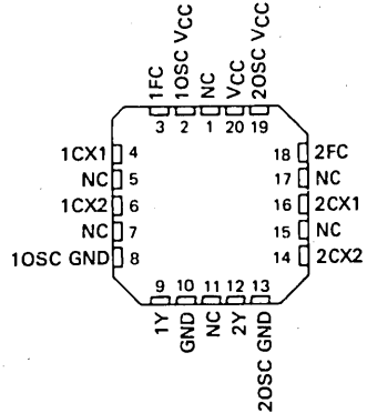
SN54LS628 ... FK PACKAGE SN74LS628 ... FN PACKAGE (TOP VIEW)
