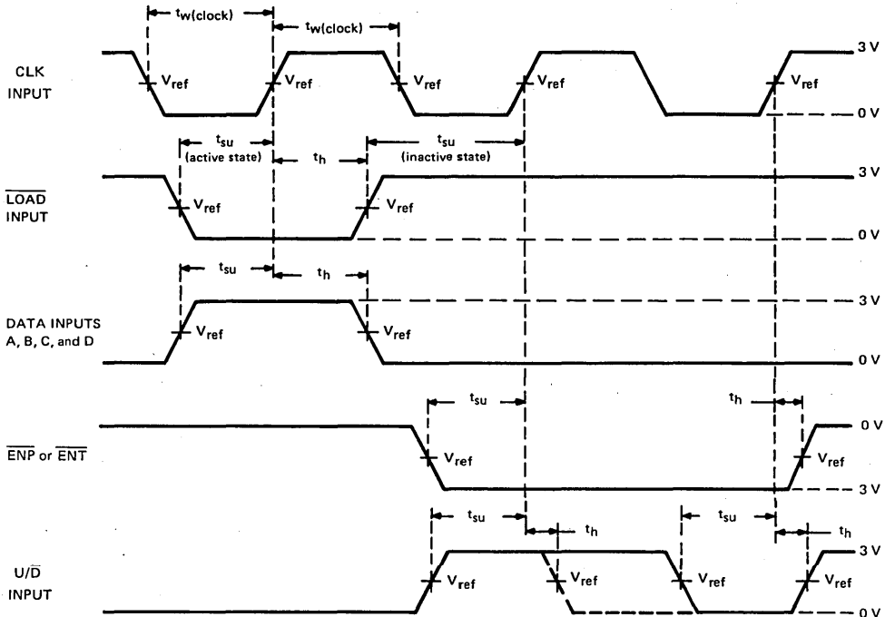
VOLTAGE WAVEFORMS
