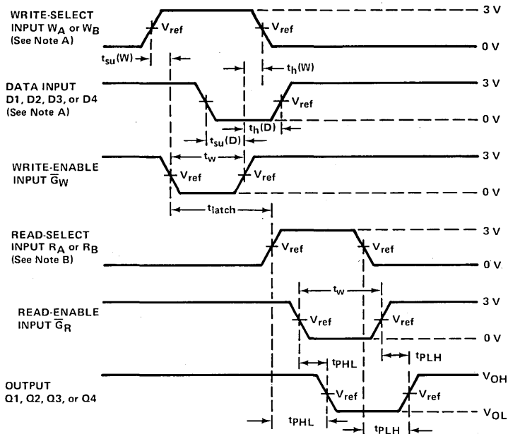
VOLTAGE WAVEFORMS
