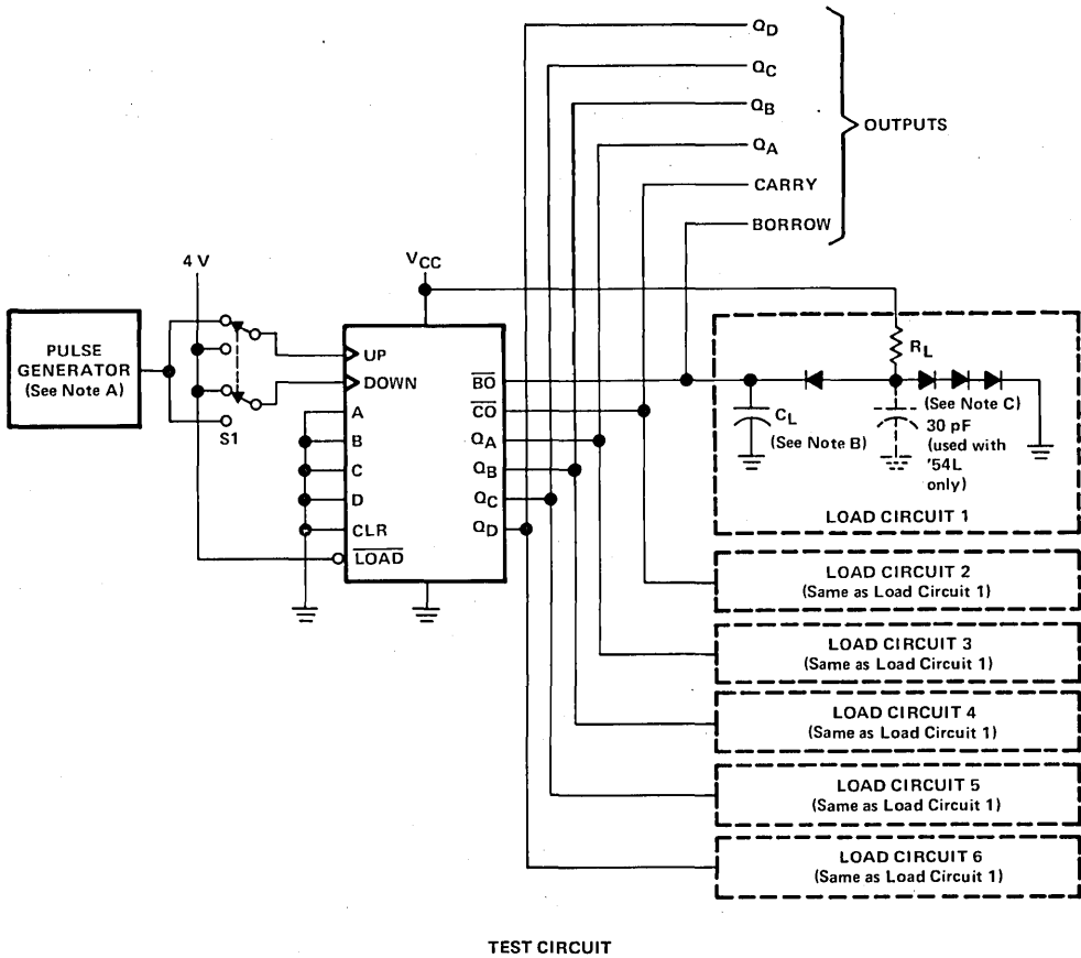
TEST CIRCUIT
