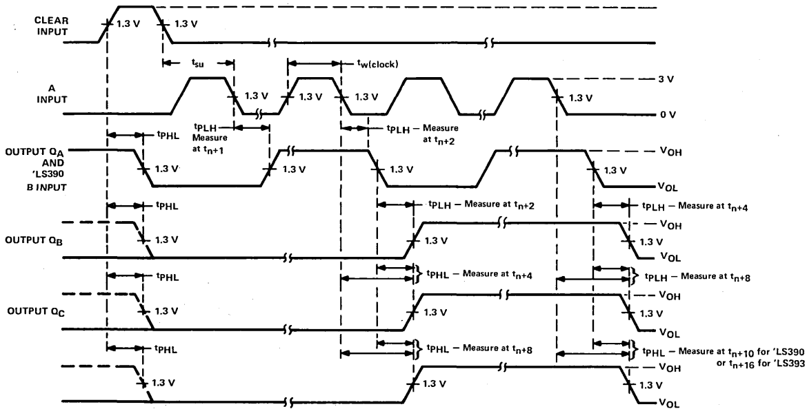
VOLTAGE WAVEFORMS
