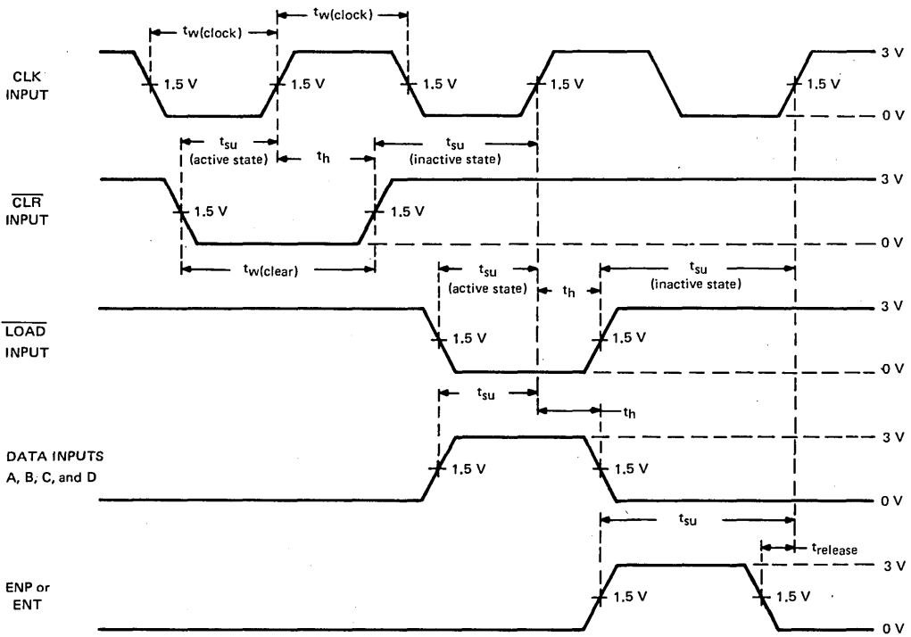
VOLTAGE WAVEFORMS
