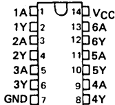
SN74LS24 ... D, J OR N PACKAGE
