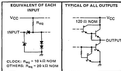
schematics of inputs and outputs
