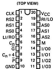
SN54LS681 ... J PACKAGE SN74LS681 ... DW, J OR N PACKAGE
