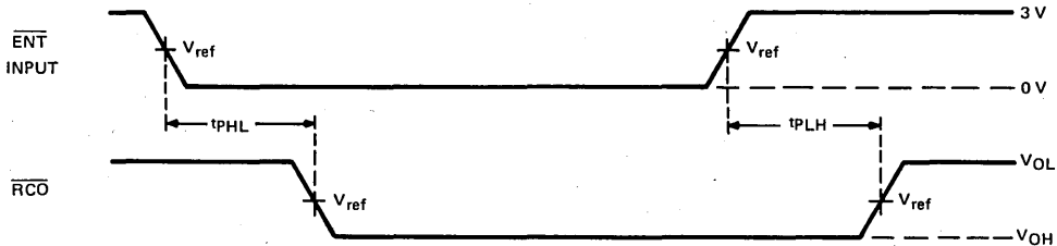
VOLTAGE WAVEFORMS
