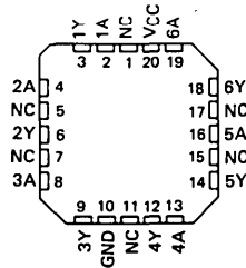
SN74LS24 ... FN PACKAGE
