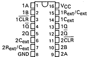
SN54LS423 ... J OR W PACKAGE SN74LS423 ... D, J OR N PACKAGE (TOP VIEW) (SEE NOTES 1 THRU 4)
