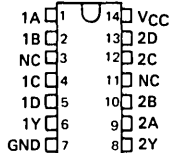
SN74LS18 ... FN PACKAGE
