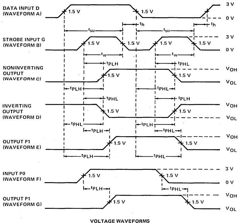
FIGURE 1—SWITCHING TIMES
