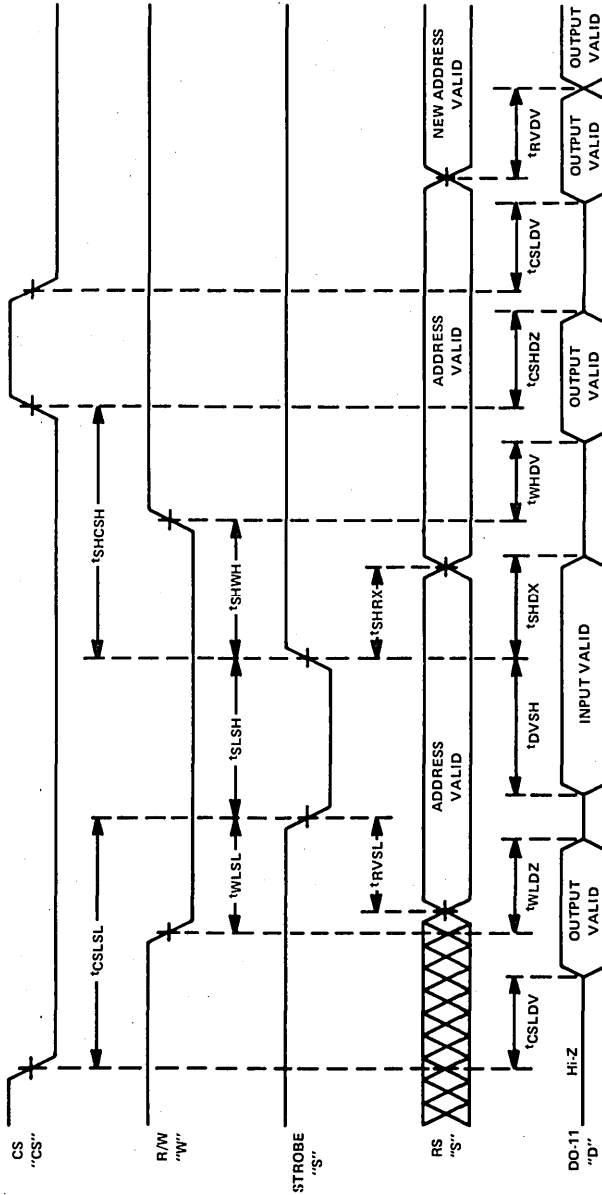
FIGURE 1—WRITE AND READ MODES
