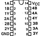
SN74LS24 ... D, J OR N PACKAGE
