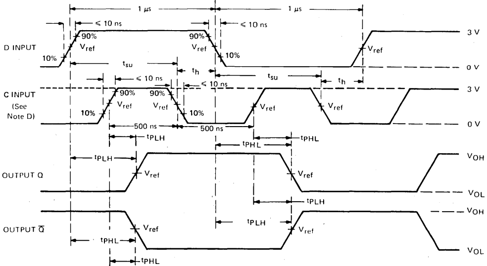
VOLTAGE WAVEFORMS
