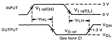
VOLTAGE WAVEFORMS
