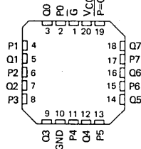
SN54LS688, SN54LS689 . . . FK PACKAGE SN74LS688, SN74LS689 . . . FN PACKAGE (TOP VIEW)
