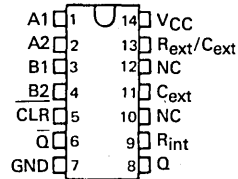
SN54LS422 ... J OR W PACKAGE SN74LS422 ... D, J OR N PACKAGE (TOP VIEW) (SEE NOTES 1 THRU 4)
