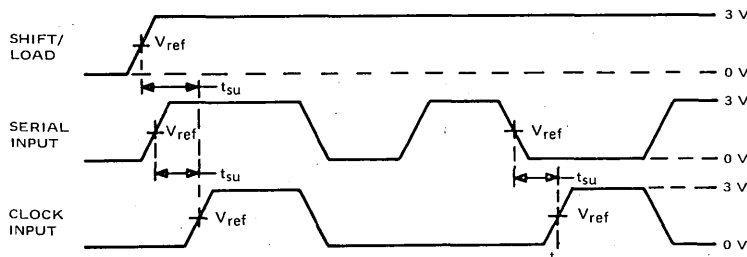
FIGURE 1—VOLTAGE WAVEFORMS
