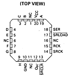
SN54LS597 ... FK PACKAGE SN74LS597 ... FN PACKAGE
