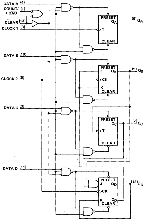
SN54176, SN74176
