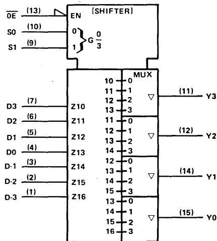
logic symbol
