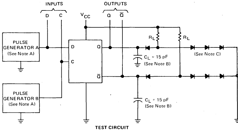
TEST CIRCUIT
