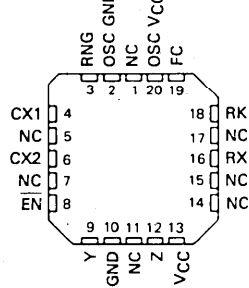
SN54LS629 ... FK PACKAGE SN74LS629 ... FN PACKAGE (TOP VIEW)
