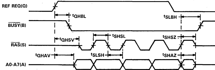
FIGURE 1 - TRANSPARENT REFRESH
