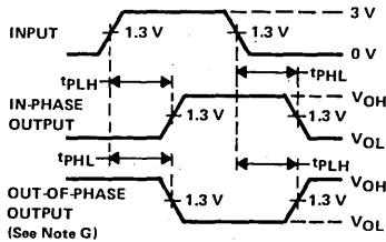
VOLTAGE WAVEFORMS PROPAGATION DELAY TIMES
