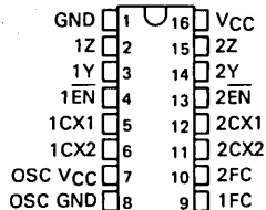
SN54LS626 ... J OR W PACKAGE SN74LS626 ... D, J OR N PACKAGE (TOP VIEW)
