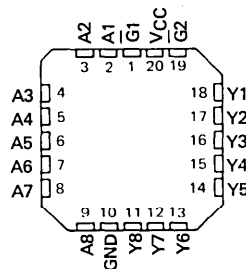
SN54LS540, SN54LS541 ... FK PACKAGE SN74LS540, SN74LS541 ... FN PACKAGE (TOP VIEW)
