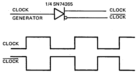
FIGURE B - SKEWLESS CLOCK/CLOCK GENERATOR CIRCUIT
